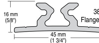
2720 Small Boat traveler track
