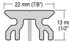
3807 Slug-mount track
