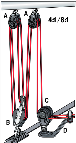
4:1/8:1 Swivel Base: Similar to the 3:1/6:1 swivel base system, but uses a 4:1/8:1 tackle for more power.
