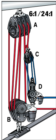
6:1 / 24:1 Cascaded: This 6:1 / 24:1 system is used on boats with mains as large as 25.5 m 2 (275 ft 2 ) and end-boom sheeting.
