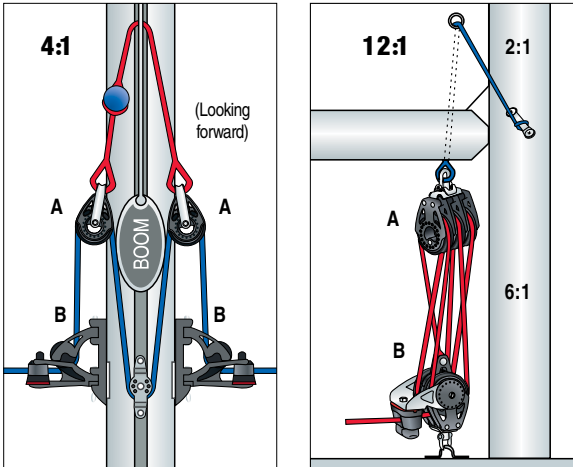
4:1 Double-ended Cascaded: This system is easy to adjust from the trapeze. It's easy to rig and unrig. Popular on smaller beachcats. 12:1 Cascaded: This simple 2:1 purchase is attached to a 6:1 cascade for a 12:1 system. Used on larger racing and cruising boats.
