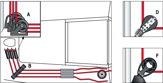
3 Halyards: Larger boats use special mastbase halyard lead blocks. Lines are routed out to deck organizers then aft to stoppers and winches. Stand-up blocks on a base are sometimes preferred for their complete articulation, but they hold halyards higher off the deck than specialized mastbase blocks.
