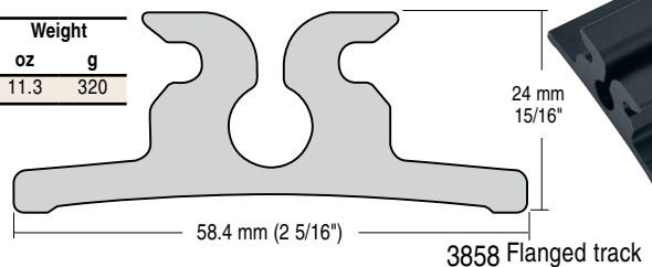
3858 Flanged track
