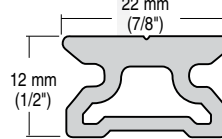
2720 Small Boat traveler track
