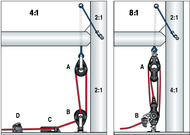
4:1 Cascaded: This simple 4:1 system leads aft to the cockpit. A favorite on small keelboats and daysailers. 8:1 Cascaded: The most basic cunningham is a self-cleating 8:1 tackle positioned at the mastbase.
