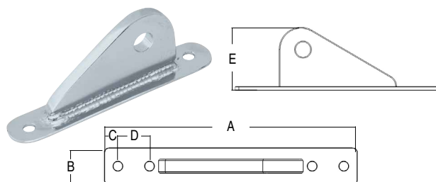
FLAT BASE BOOM FITTINGS
