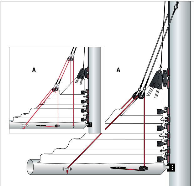
Lazy Jacks: Lazy Jacks contain mainsails during reefing and dousing. They work exceptionally well with full-battened mains, but are also used with conventional sails.
