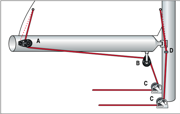
Dual Line: This dual-line system is common on boats 9 m (30') and larger. Position blocks so line pulls down and out to keep the sail flat and prevent lateral loads on the luff rope or luff sliders.
