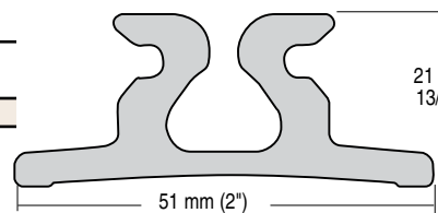
3849 Flanged track
