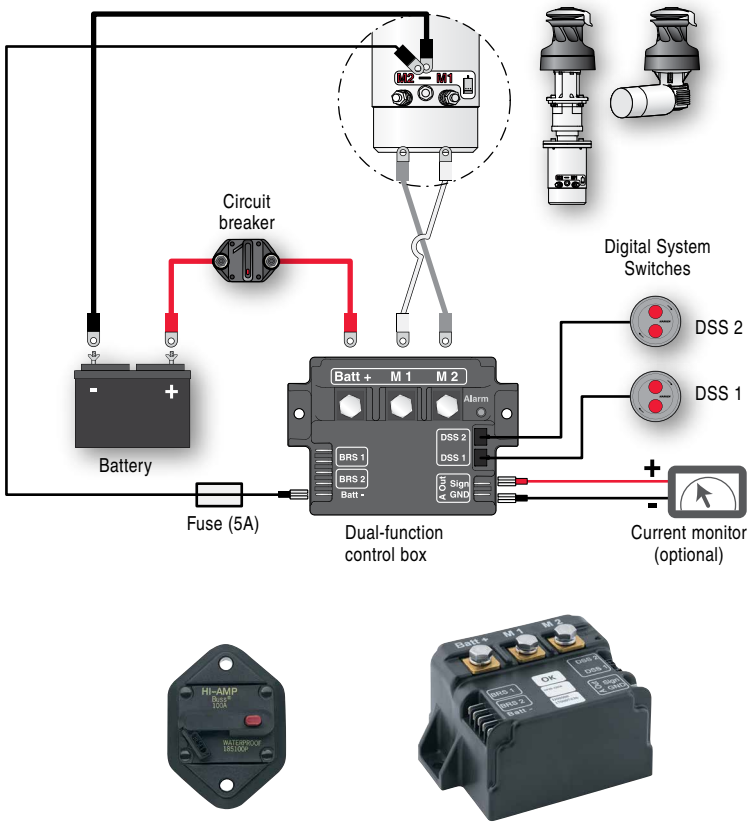
CIRCUIT BREAKERS
