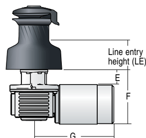
ELECTRIC HORIZONTAL
