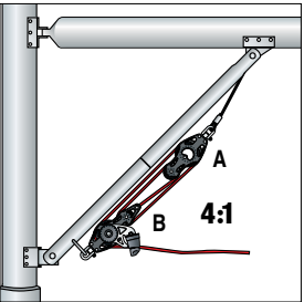
4:1 Cascaded Kicker: This rigid rod vang utilizes a simple 4:1 tackle. The rod also serves as a topping lift for the boom. Used on cruising and racing boats.
