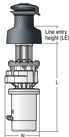
ELECTRIC VERTICAL
