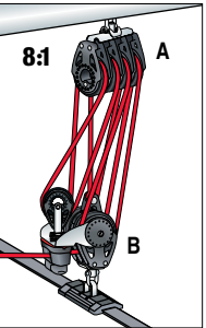
8:1 Beachcat: This 8:1 purchase handles high mainsheet loads on Beachcats up to 6 m (20').
