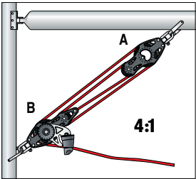
4:1 Fiddle: The basic 4:1 fiddle block vang is commonly used on dinghies and small keelboats.
