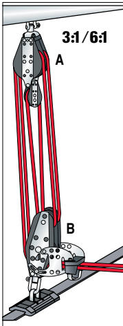
3:1/6:1: This 3:1/6:1 two-speed system is used on end-boom sheeting and mainsails up to 22.3 m² (240 ft²).
