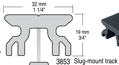
3853 Slug-mount track
